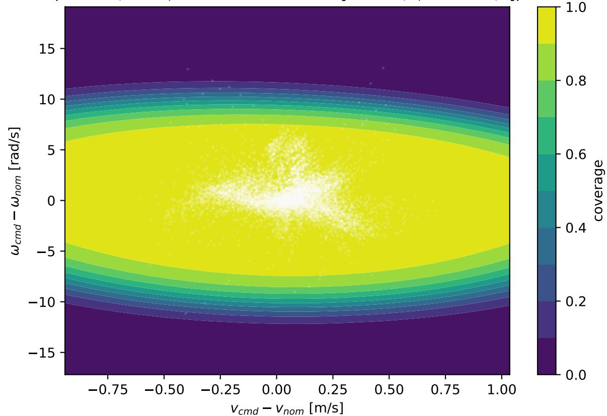
Residual coverage vs command offset (0 = off / OOD; state fixed at mean [0.55 m/s, 0.49 rad/s])
